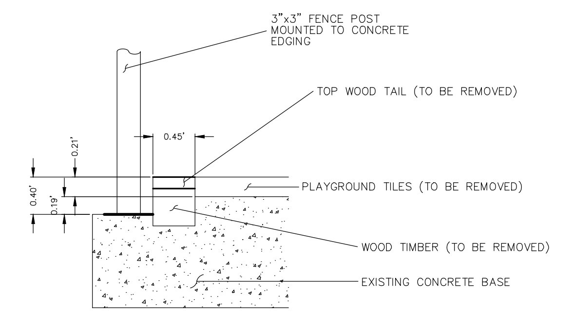
EXISTING SECTION DETAIL NOT TO SCALE
