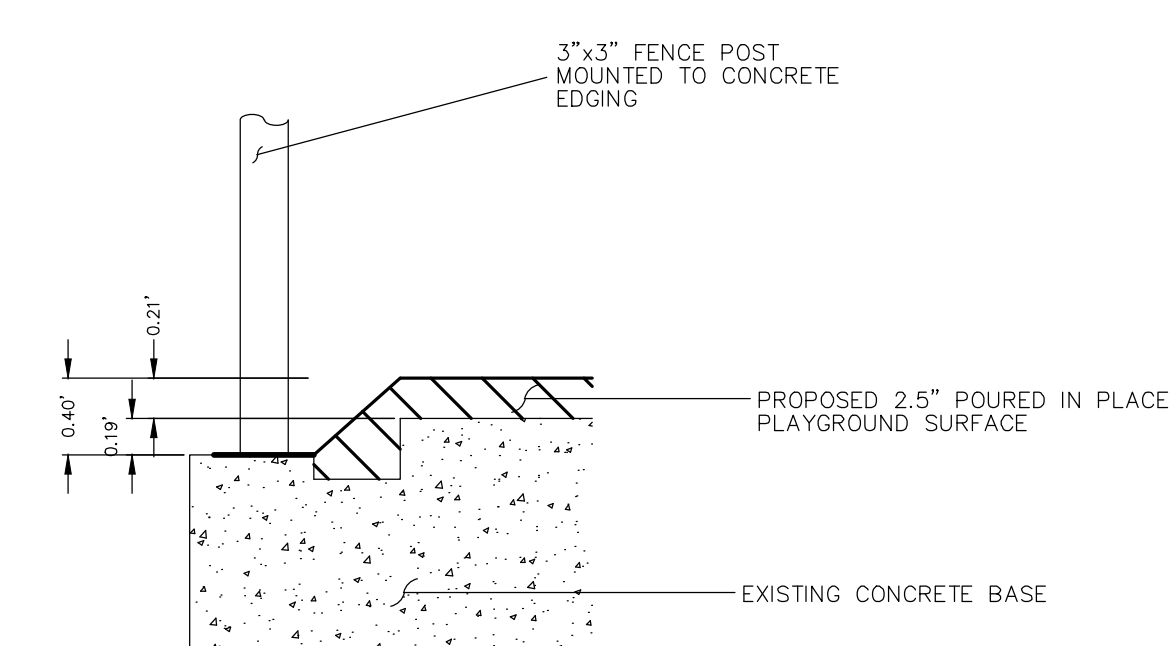
PROPOSED TYPICAL SECTION DETAIL NOT TO SCALE
